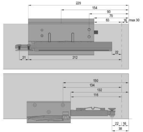
Mechanism mounting dimensions / External door
