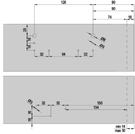
Mechanism mounting dimensions / Internal door
